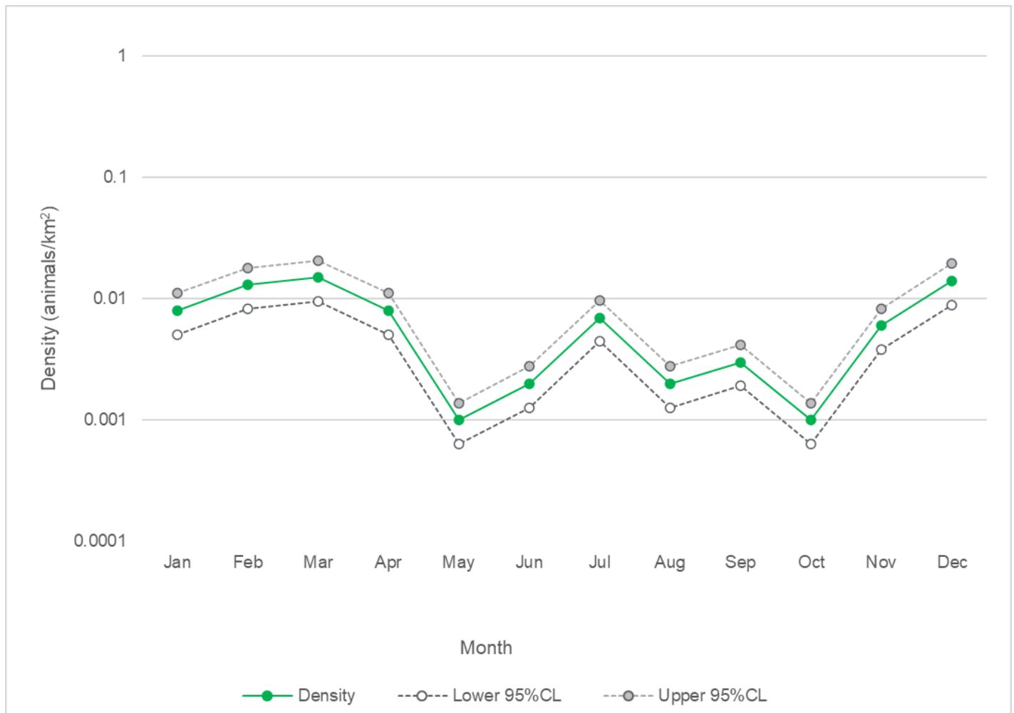
Figure A.21: Estimated monthly mean relative density of grey seal over the Mona Aerial Survey Area, with lower and upper confidence limits.
