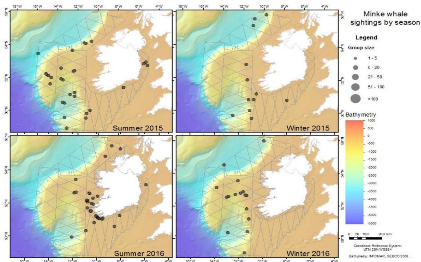
Figure 1.61: Sightings of minke whales in each survey period (bottom). Grey lines indicate the survey track lines along which sightings were made. Circles are proportional to the number of individuals in each sighting. From Rogan et al. (2018).
